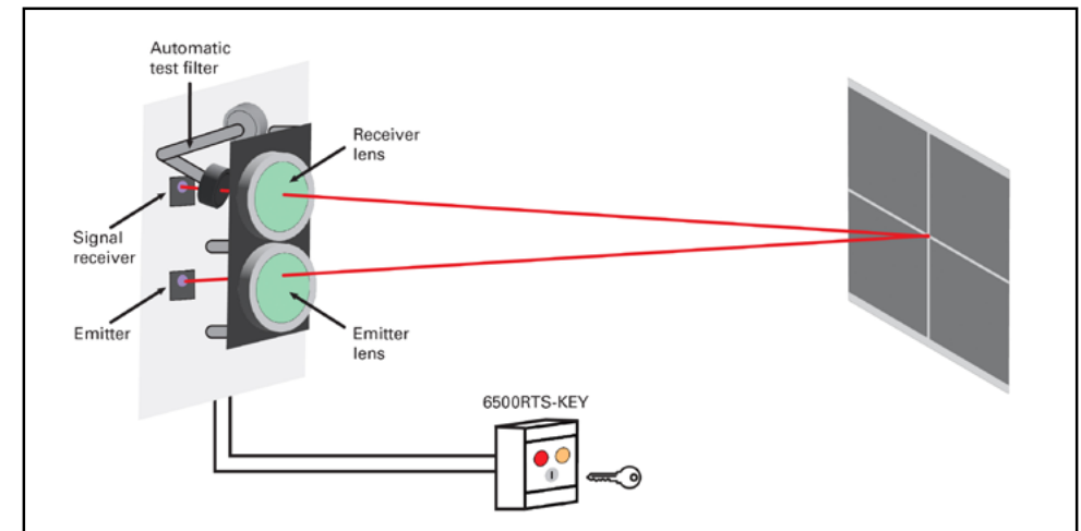
Notifier Opal Beam Detector remote test operation
