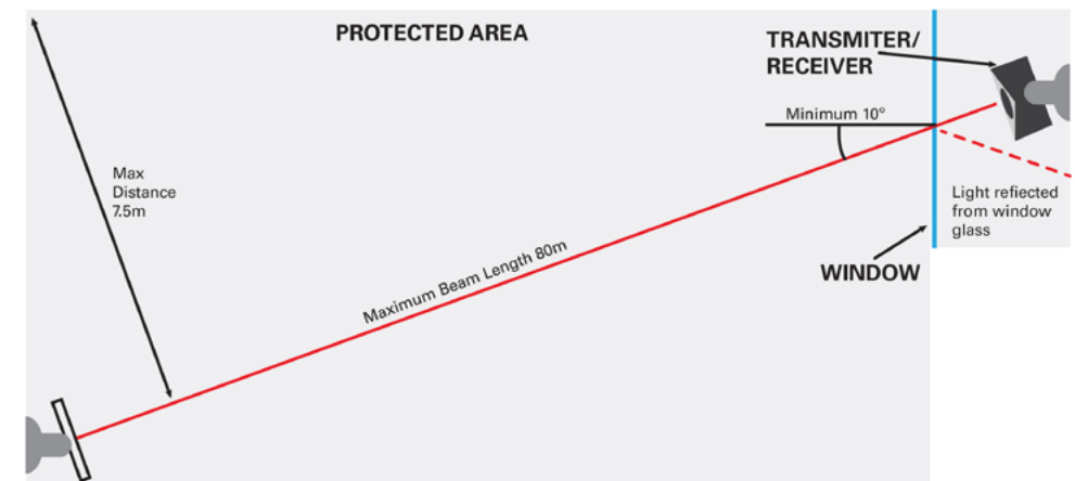
Reflective Beam Detector Operating through a Window
